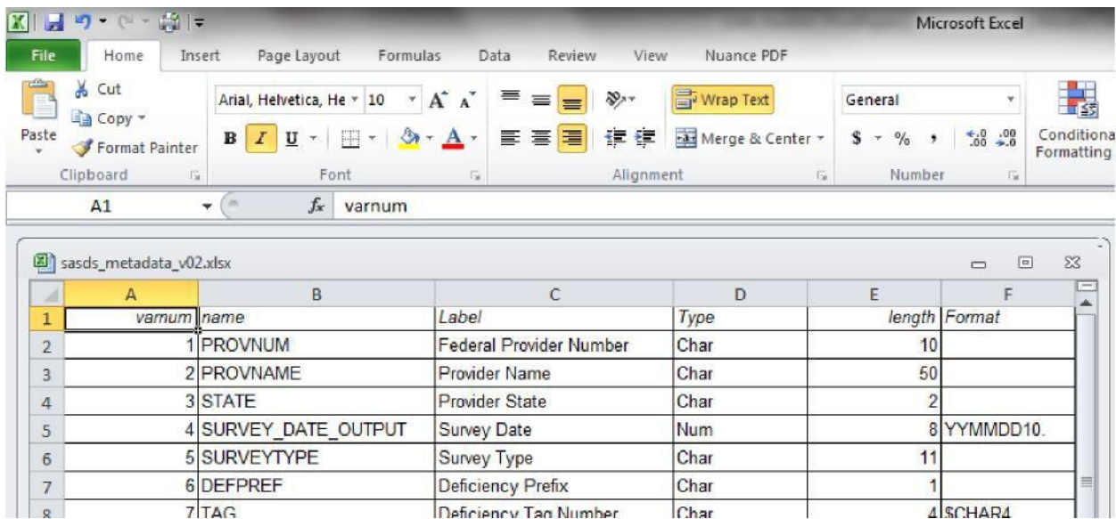
Figure 15. Generation of Excel Documentation – File Documentation tab
