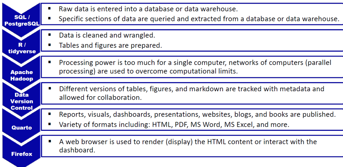
Figure 1. The Open Source workflow of a data scientist.
