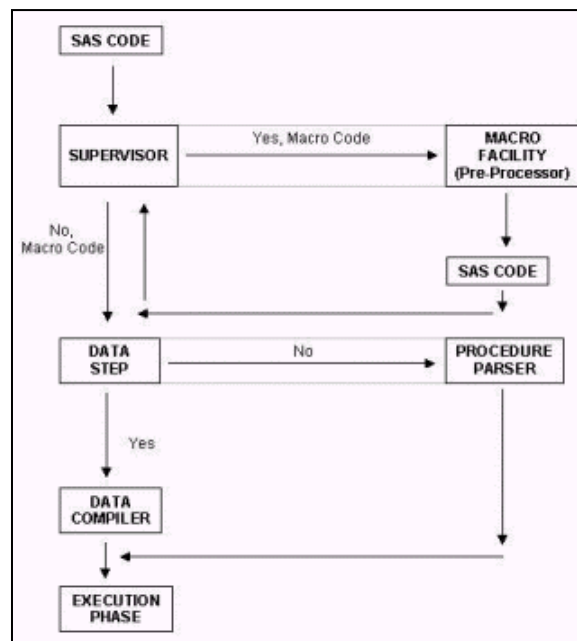
Figure 1. Macro Program Control Flow.
