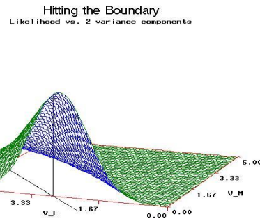
Figure 3. Boundary problems in random effects models.
