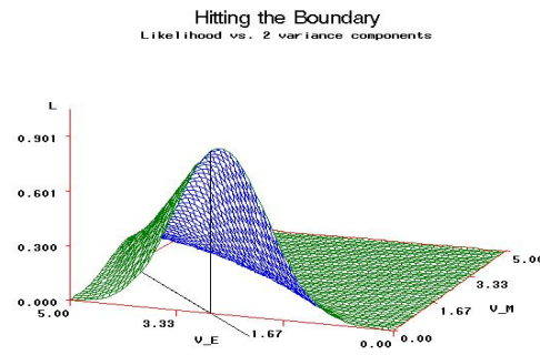
Figure 3. Boundary problems in random effects models.
