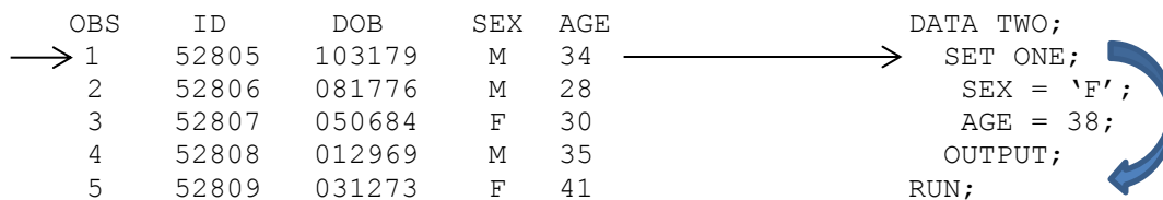
Figure 1. SAS data set ONE
