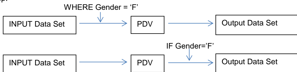
Figure 10. WHERE and IF along the Observation Loop.
