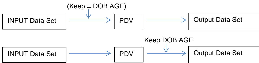
Figure 20. KEEP/DROP and the observation loop
